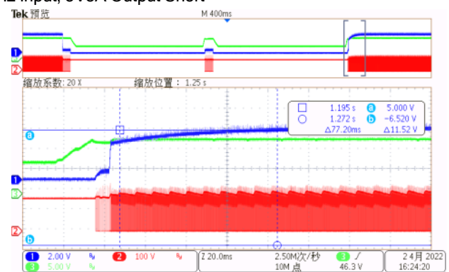
(CH1-Vo, CH2-VDrain, CH3-VDDL) Comments: Recover to 5V
