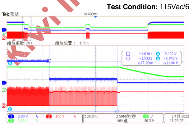
(CH1-Vo, CH2-VDrain, CH3-VDDL) Comments: Protection enter
