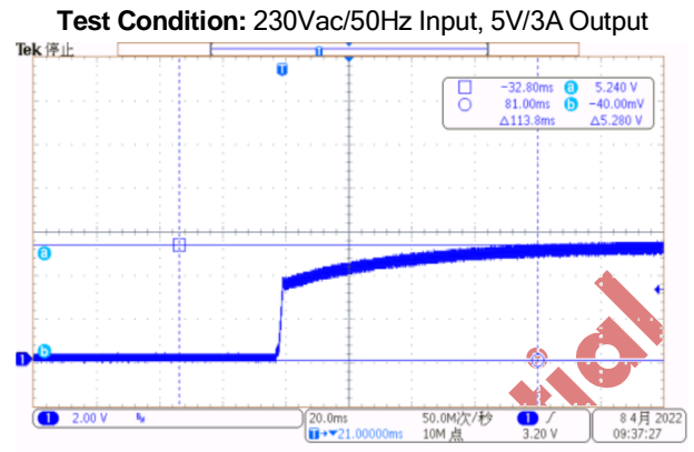
(CH1- Vo) Comments: Vo-peak=5.24V
