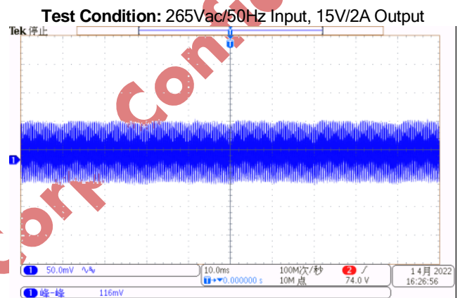
(CH1- Ripple) Comments: Vripple=116mV
