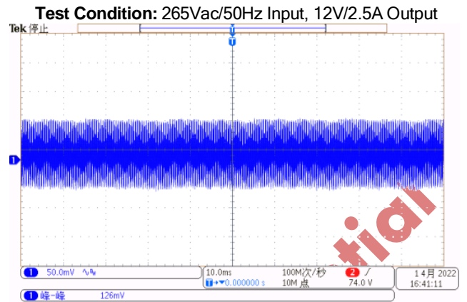
(CH1- Ripple) Comments: Vripple=126mV
