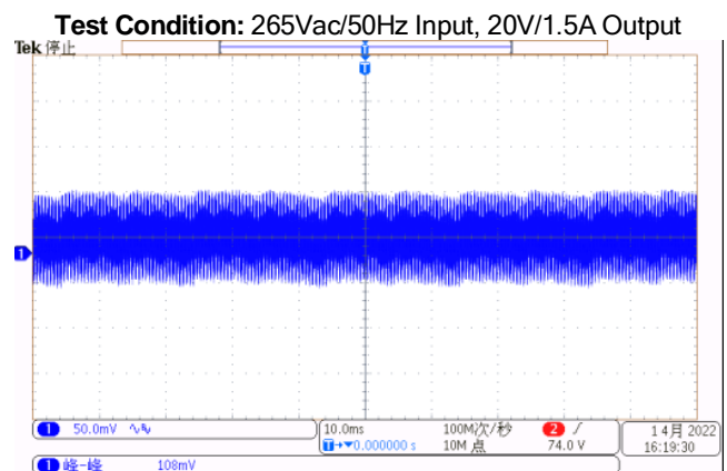
(CH1- Ripple) Comments: Vripple=108mV
