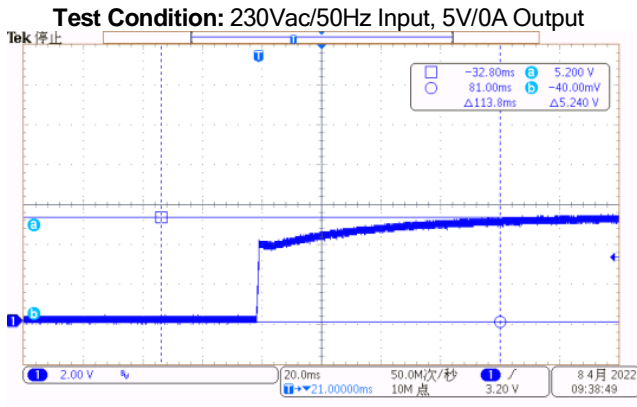
(CH1- Vo) Comments: Vo-peak=5.2V
